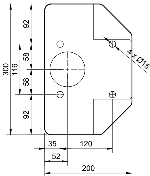
Detail "X": Bodenmontage M 1:5
